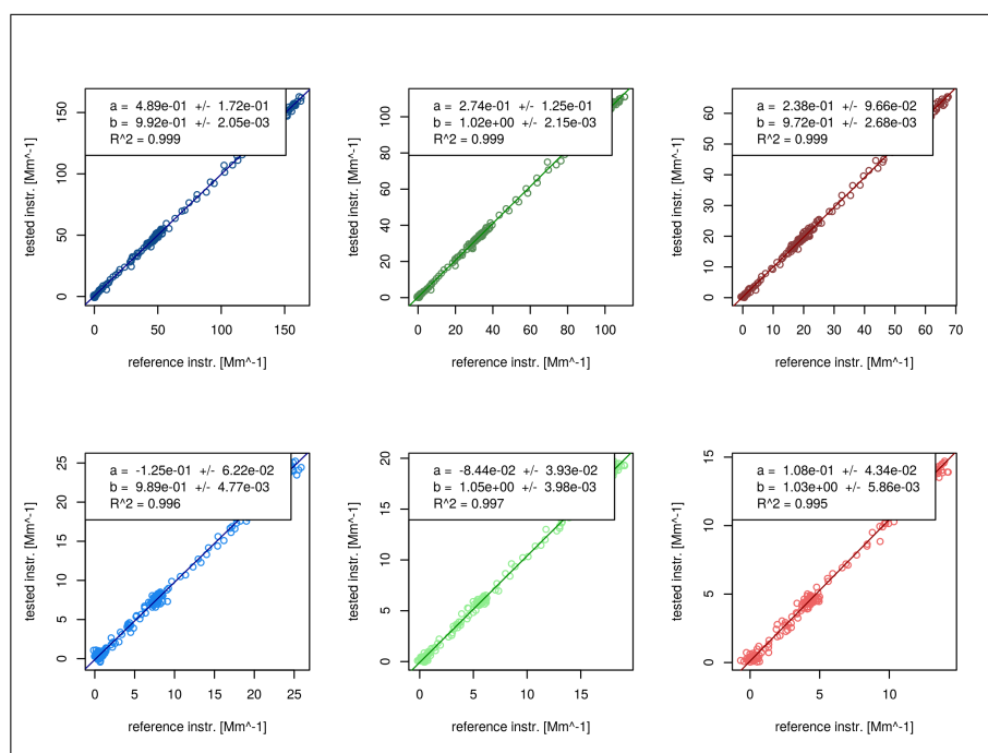
Figure 1: Correlation of scattering coefficients from nephelometer (SN 70919196) and reference nephelometer Aurora4000 (SN 14-1408) before inspection and recalibration. Testaerosol is ammonium sulfate.
