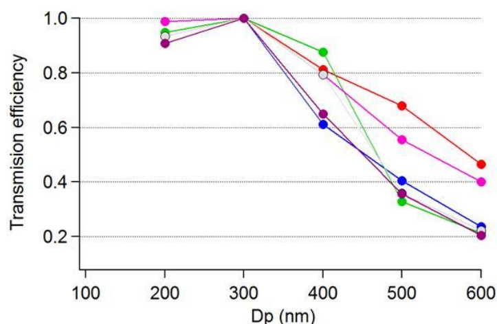
Figure 3.1 Transmission efficiency measured for five different instruments from diameters of 200 nm up to 600 nm.
