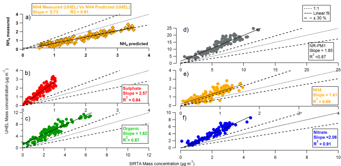
Figure 4.3. a) \text{NH}_4 measured vs \text{NH}_4 predicted for UHEL instrument, and comparison of the UHEL instrument with the Sirta instrument for b) \text{SO}_4 , c) Org, d) Total NR-PM1 mass concentration, e) \text{NH}_4 , and f) \text{NO}_3 .
