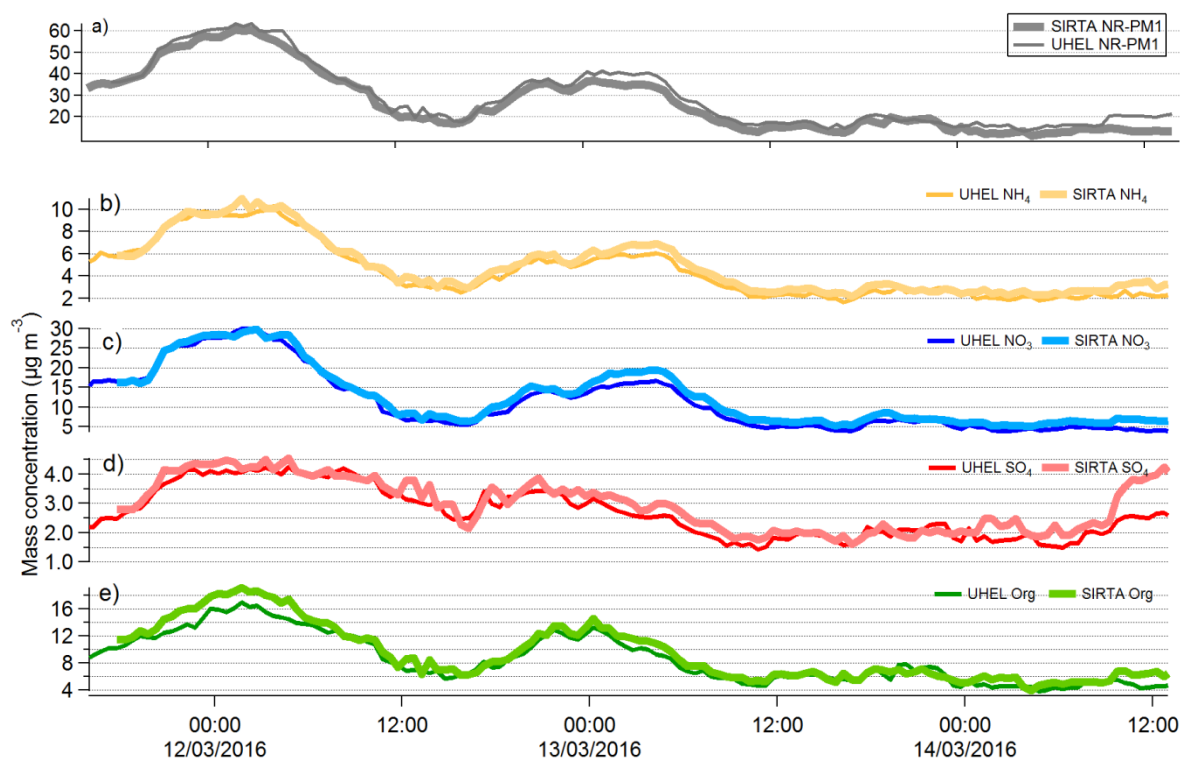
Figure 5.1. Comparison of UHEL with reference instrument for a) Total PM, b) Ammonia, c) Nitrate, d) sulphate, and e) Organic.
