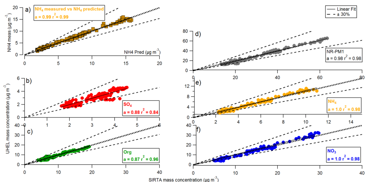
Figure 5.2. a) \text{NH}_4 measured vs \text{NH}_4 predicted for UHEL instrument, and comparison of the UHEL instrument with the Sirta instrument for b) \text{SO}_4 , c) Org, d) Total NR-PM1 mass concentration, e) \text{NH}_4 , and f) \text{NO}_3 .
