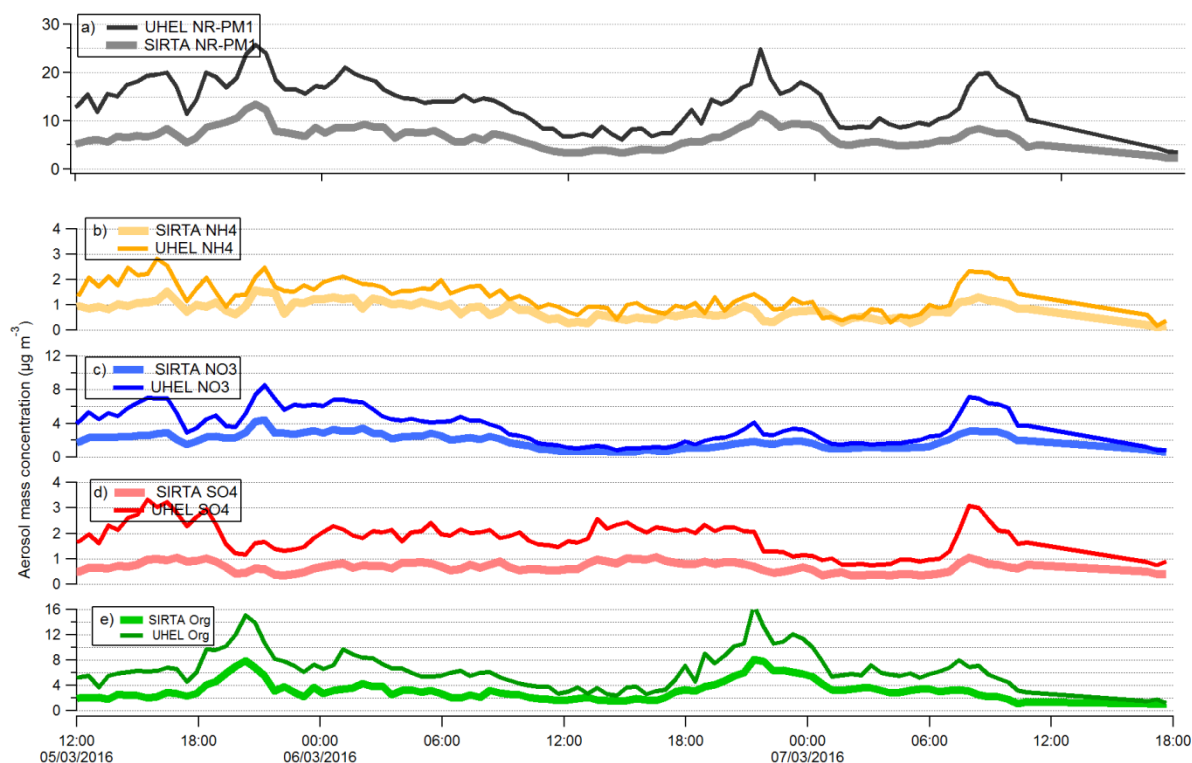
Figure 4.2. Comparison of a) total NR-PM1 mass concentration and of each of the individual species measured by the ACSM, as well as the individual chemical species b) \text{NH}_4 , c) \text{NO}_3 , d) \text{SO}_4 , e) Org.
