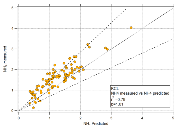
Figure 3.2 \text{NH}_4 measured vs \text{NH}_4 predicted for the KCL instrument (24/11 00hrs to 26/11 00hrs) using the calibrated RIE \text{NH}_4 values listed in Table 3.2.
