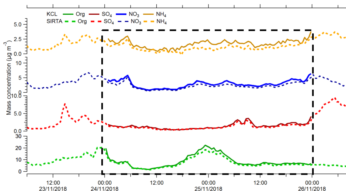
Figure 4.1. Comparison of KCL with SIRTa instrument for Ammonia, Nitrate, sulphate, and organic, during the second intercomparison campaign. The highlighted box indicates the intercomparison period (24/11 00hrs to 26/11 00hrs).
