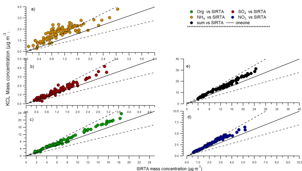
Figure 4.2. Correlations between different chemical species measured by the KCL and the SIRTa instrument during the second intercomparison campaign (24 th Nov 00hrs to 26 th Nov 00hrs).
