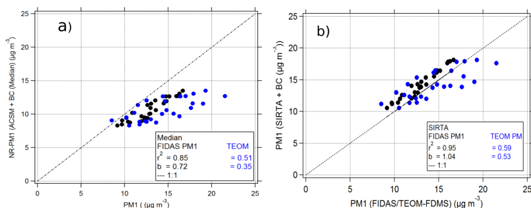
Figure 2.2. Comparison of a) Robust Median PM1 and b) SIRTAs NR-PM1 + BC mass concentrations with those of the FIDAS and TEOM PM1 mass concentration.
