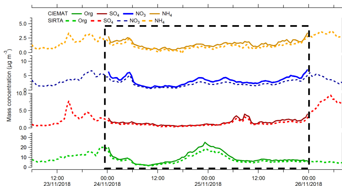
Figure 4.1. Comparison of CIEMAT with SIRTa instrument for Ammonia, Nitrate, sulphate, and organic, during the second intercomparison campaign. The highlighted box indicates the intercomparison period (24/11 00hrs to 26/11 00hrs).
