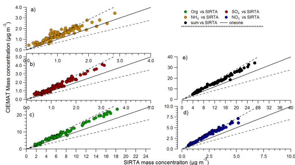
Figure 4.2. Correlations between different chemical species measured by the CIEMAT and the SIRTa instrument during the second intercomparison campaign (24 th Nov 00hrs to 26 th Nov 00hrs).
