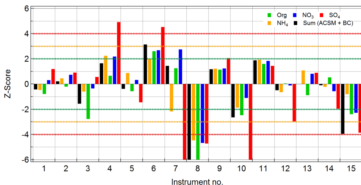
Figure 2.1. Z-score calculation for each species measured by the ACSM for each instrument that participated in the initial intercomparison campaign (18 th Nov 18hrs to 19 th Nov 08 hrs).
