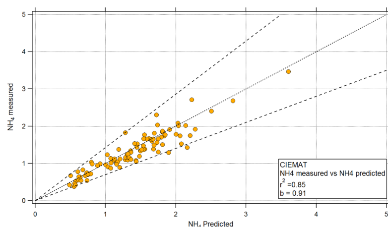
Figure 3.2 \text{NH}_4 measured vs \text{NH}_4 predicted for the CIEMAT instrument (24/11 00hrs to 26/11 00hrs) using the calibrated RIE \text{NH}_4 values listed in Table 3.2.
