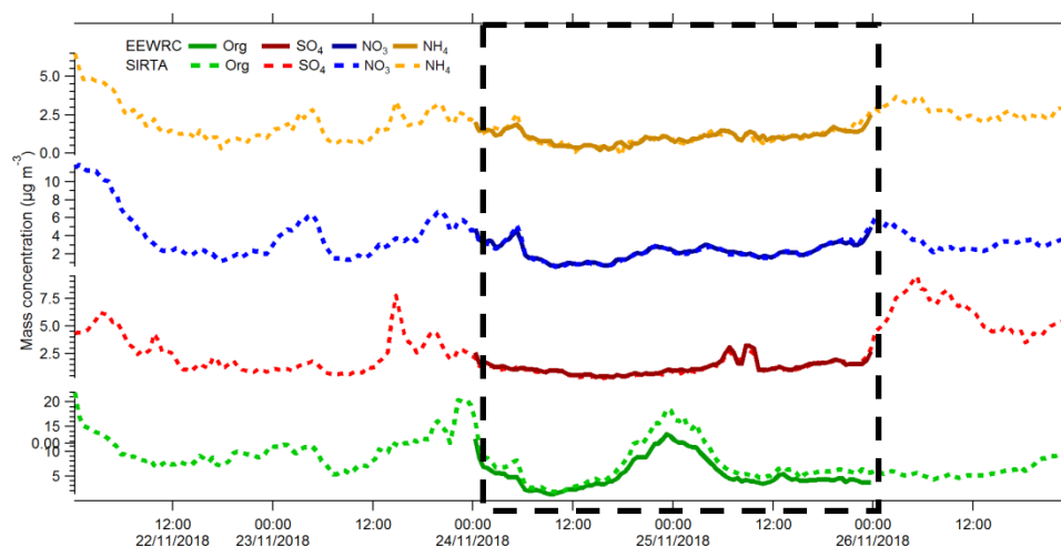
Figure 4.1. Comparison of EEWRC with SIRTa instrument and robust median data for Ammonia, Nitrate, sulphate, and organic, during the second intercomparison campaign. The highlighted box indicates the intercomparison period (24/11 00hrs to 26/11 00hrs).
