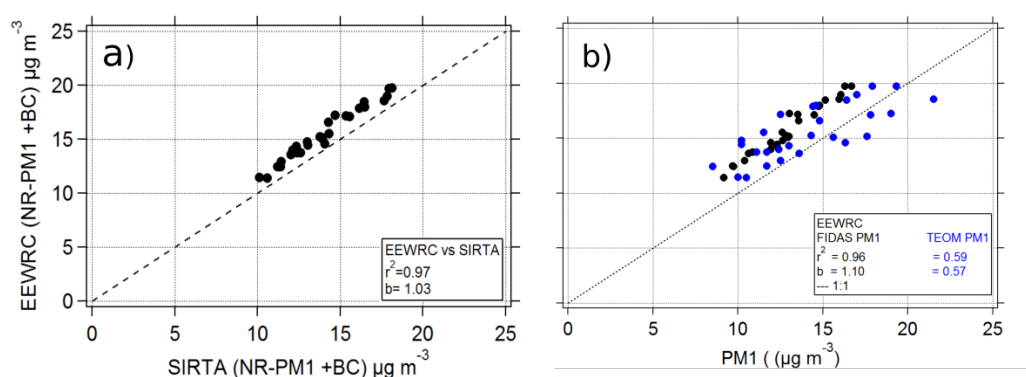
Figure 2.3. Comparison of EEWRC NR-PM1 with the a) SIRTAs NR-PM1 + BC mass concentrations and b) with PM1 mass concentration from FIDAS and TEOM PM1 mass concentration.
