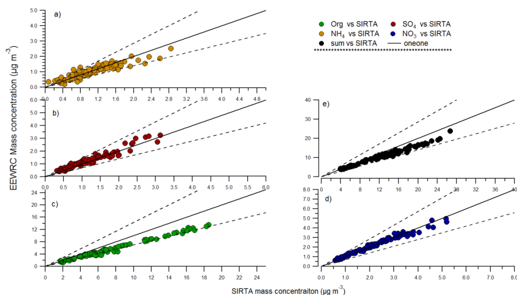
Figure 4.2. Correlations between different chemical species measured by the EEWRC and the SIRTa instrument during the second intercomparison campaign (24 th Nov 00hrs to 26 th Nov 00hrs).
