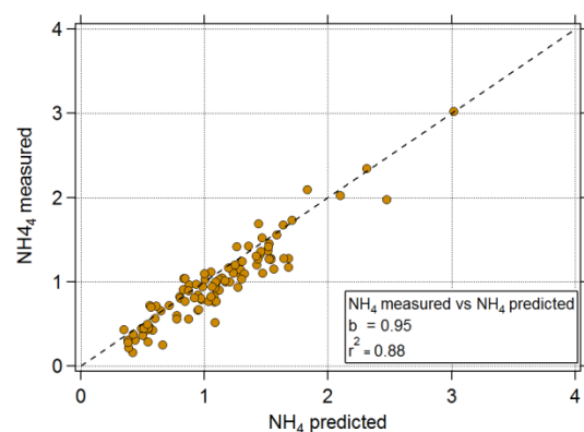
Figure 3.2 \text{NH}_4 measured vs \text{NH}_4 predicted for the EEWRC instrument using the calibrated RIE \text{NH}_4 values listed in Table 3.2.
