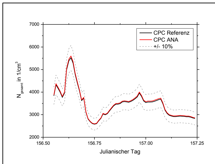
Figure 02: Inter-comparison of ambient air conditions between Reference CPC and CPC ANA.
