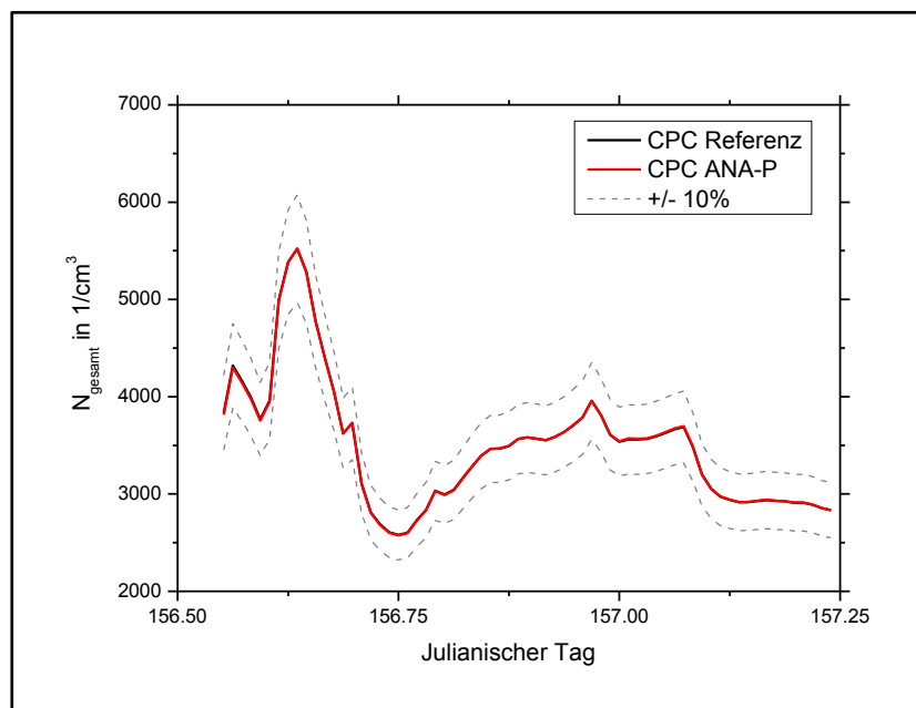
Figure 02: Inter-comparison of ambient air conditions between Reference CPC and CPC ANA-P.
