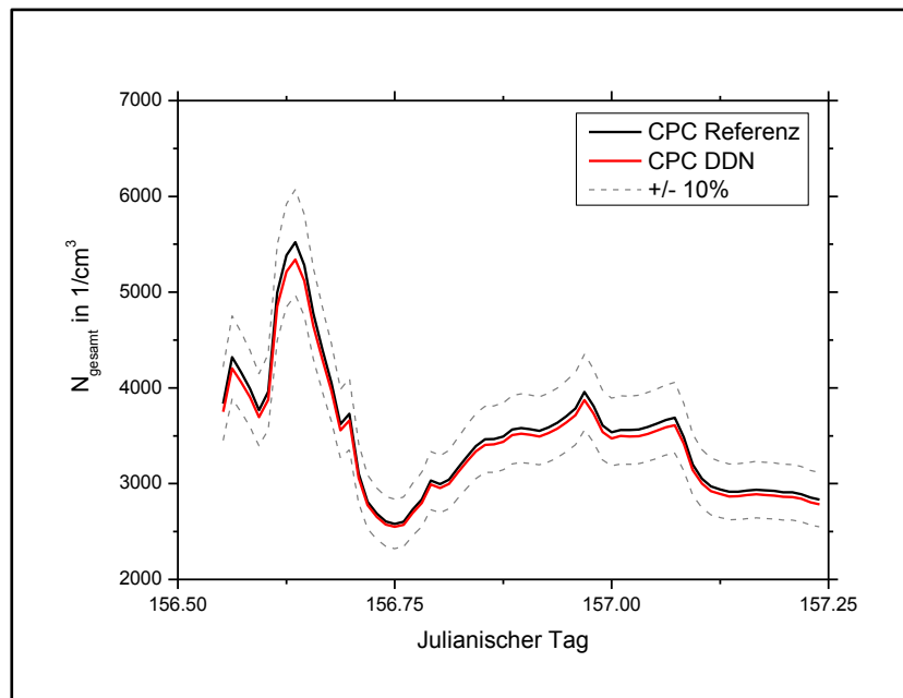
Figure 02: Inter-comparison of ambient air conditions between Reference CPC and CPC DDN.
