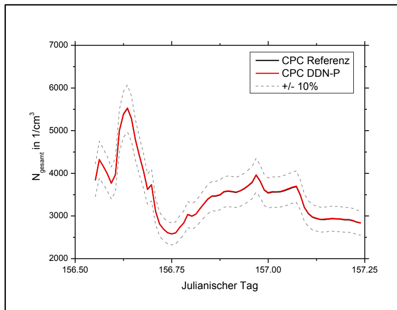
Figure 02: Inter-comparison of ambient air conditions between Reference CPC and CPC DDN-P.
