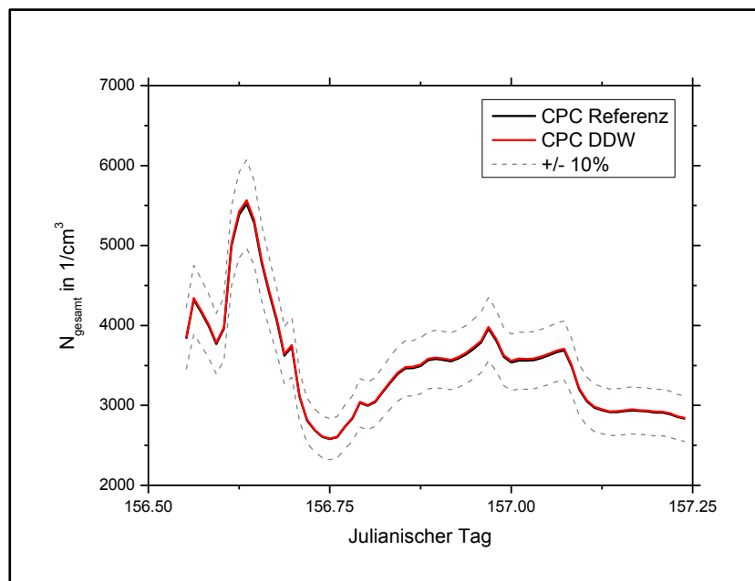
Figure 02: Inter-comparison of ambient air conditions between Reference CPC and CPC DDW.
