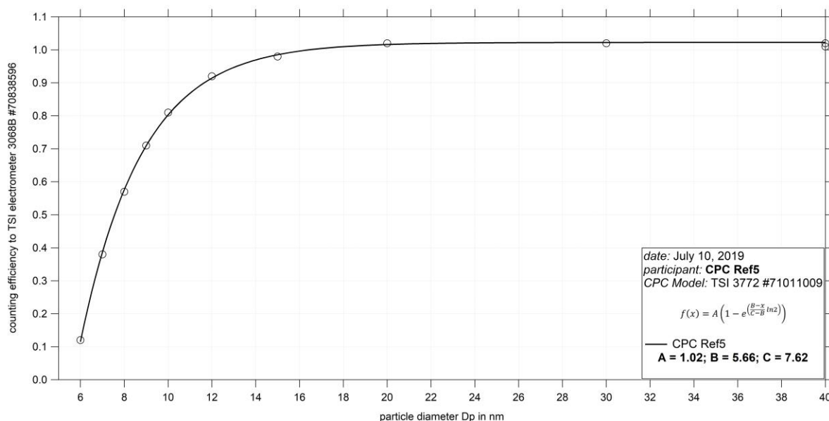
Fig. 1: Counting efficiency for CPC Ref5 3772 SN71011009 against aerosol electrometer 3068 SN 70838596; silver particles between 6 and 40 nm were used for calibration; the calculated D_{p50} is 7.62 nm.
