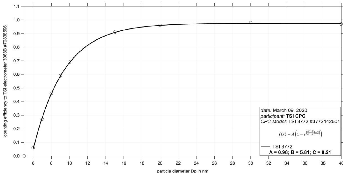
Fig. 1: Counting efficiency for CPC 3772 S/N 3772142501 against aerosol electrometer 3068 S/N 70838596; silver particles between 5 and 40 nm were used for calibration; the calculated Dp50 is 8.21 nm.
